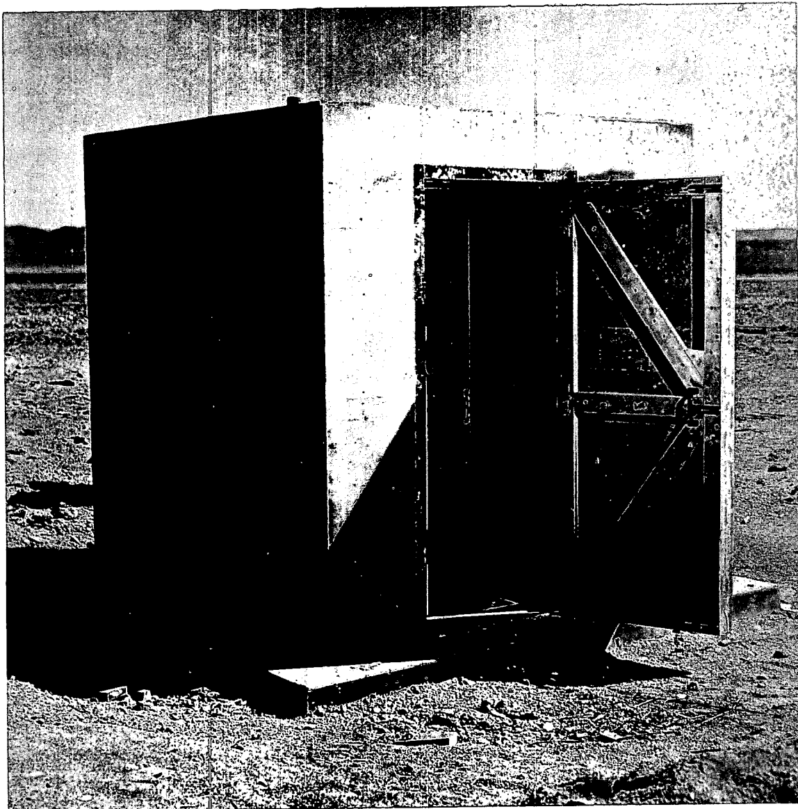
Fig. 20—Exterior of reinforced-concrete utility-type shelter, stations 1-34.1 f, i, and l.
